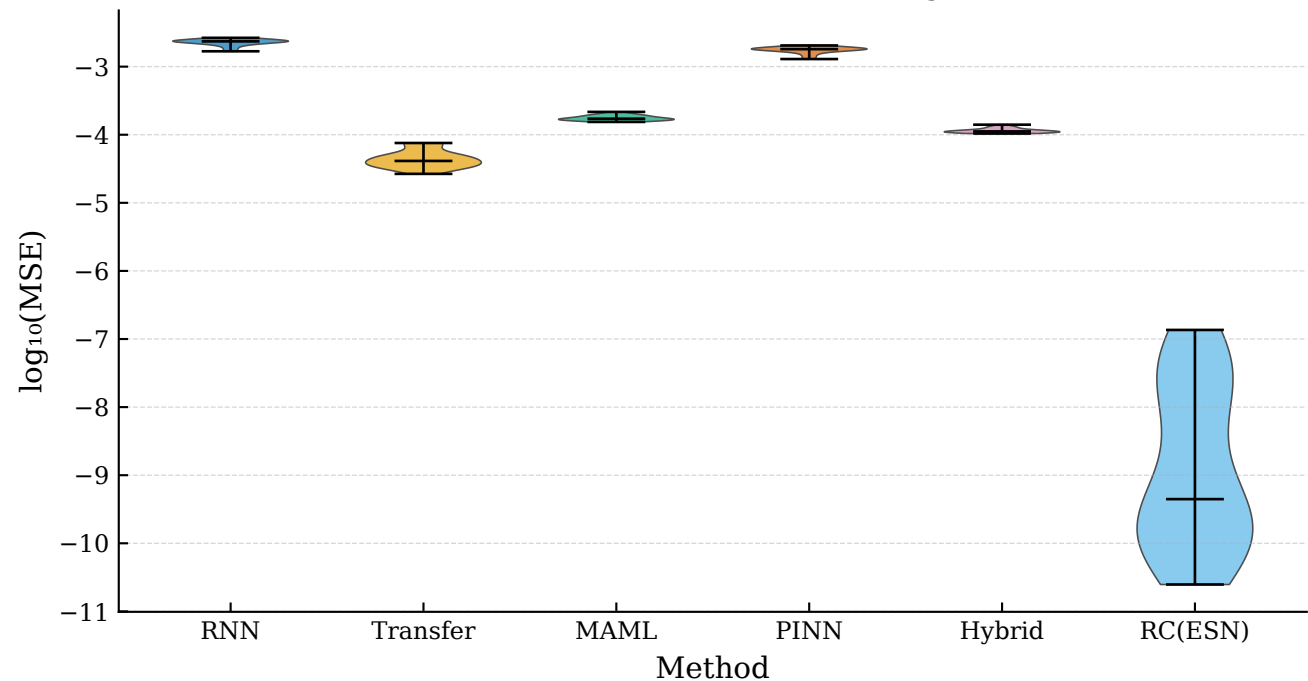
Lorenz — MSE Distribution Shape (log 10 scale)
