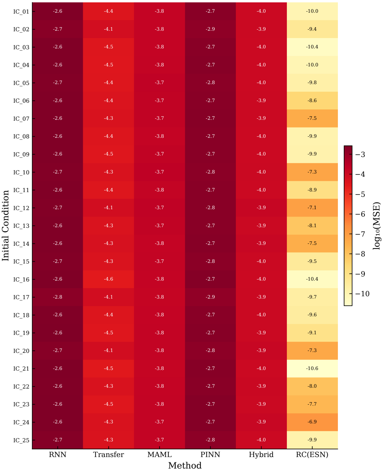
Lorenz — \log_{10}(\text{MSE}) per IC and Method
