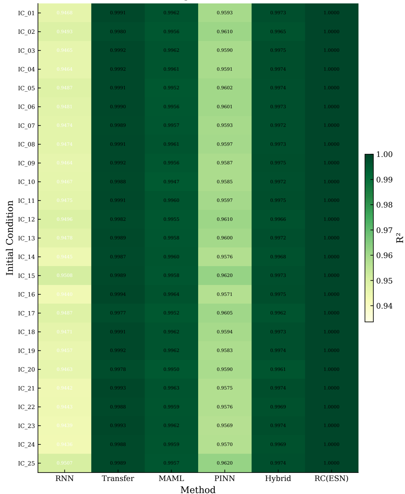
Lorenz — R 2 per IC and Method
