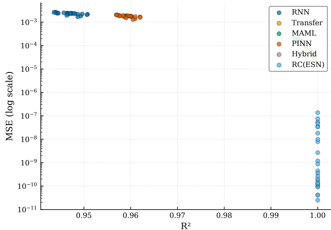
Lorenz — MSE vs R 2 for All Methods and Random ICs
