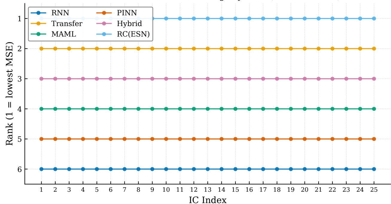
Lorenz — Per-IC Method Rankings by MSE (Rank 1 = Best)
