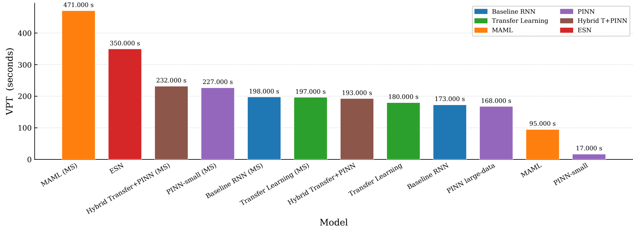
MG — Valid Prediction Time in Seconds ( \lambda_1 \approx 0.0055 ( \tau=17 ))
