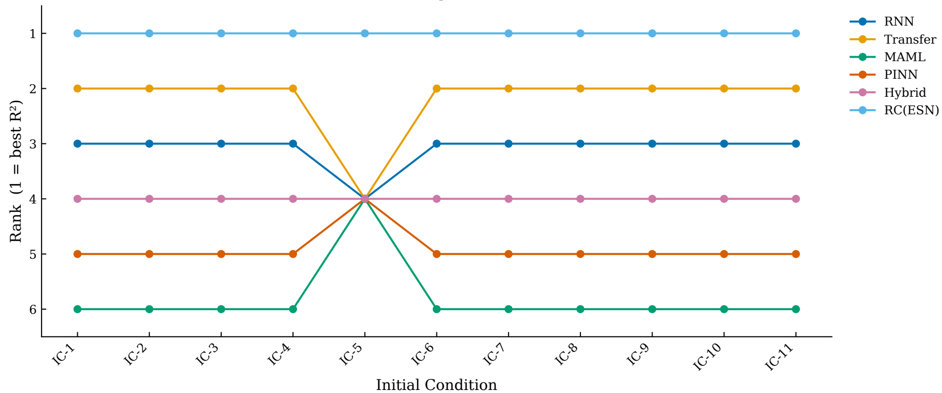
MG — Method Rank per Initial Condition
