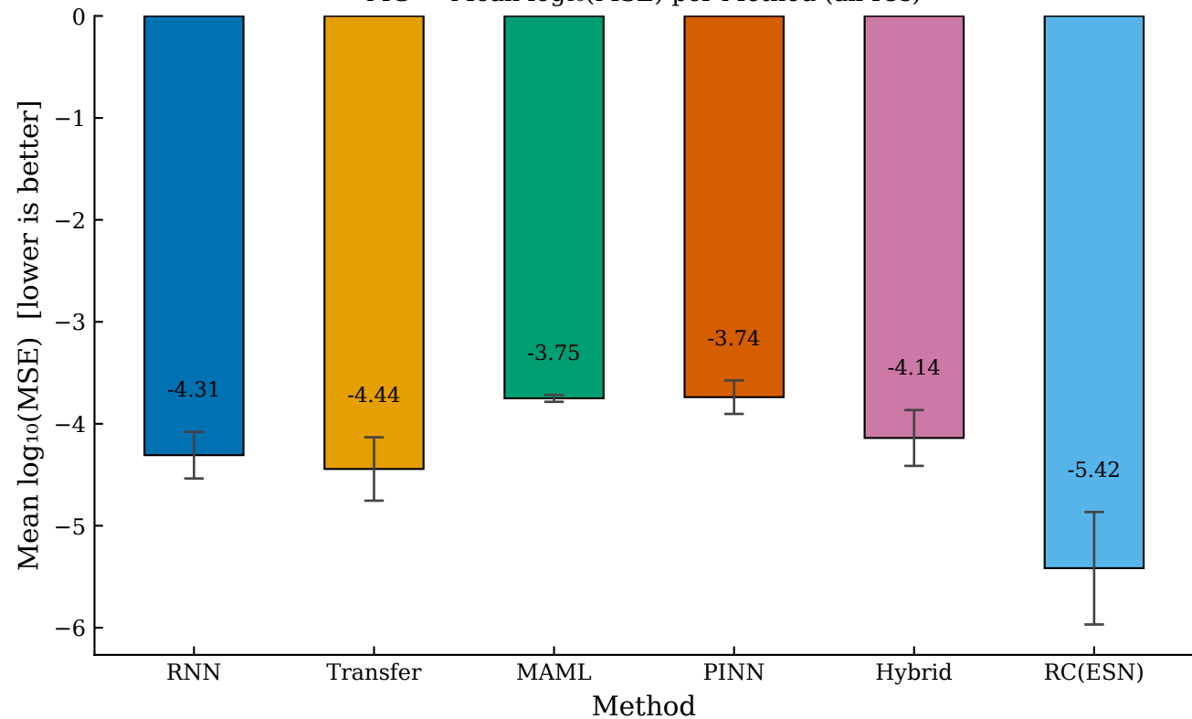
MG — Mean \log_{10}(\text{MSE}) per Method (all ICs)
