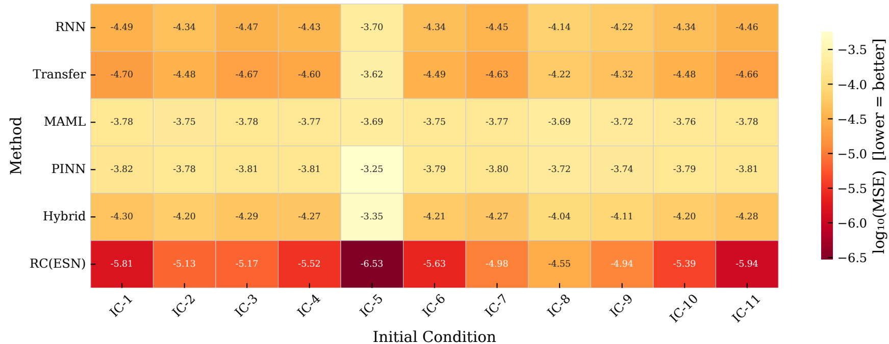
MG — \log_{10}(\text{MSE}) Heatmap: Method \times IC [lower = better]
