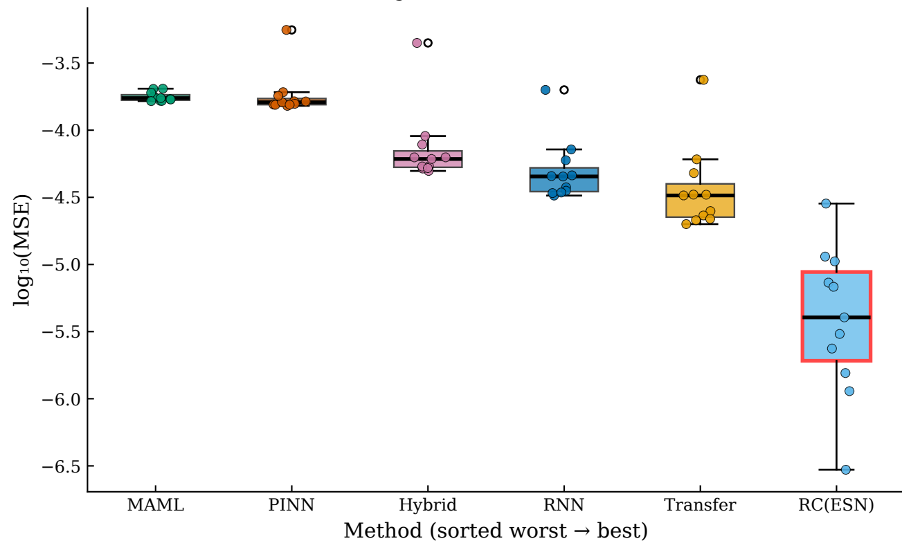
MG — \log_{10}(\text{MSE}) Distribution (all ICs)
