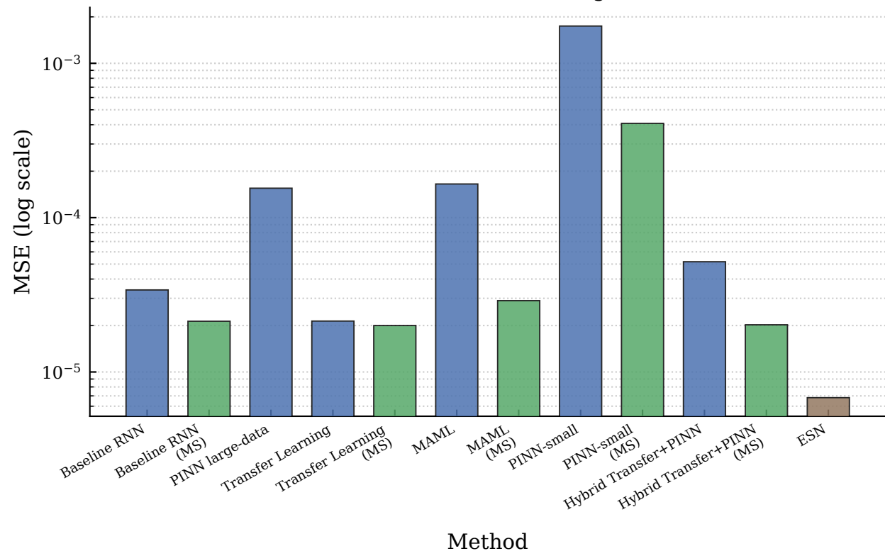
MG — MSE: All Variants (log scale)
