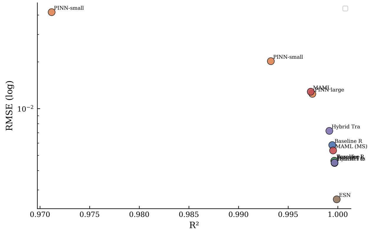
MG — RMSE vs R^2 with Pareto Frontier
