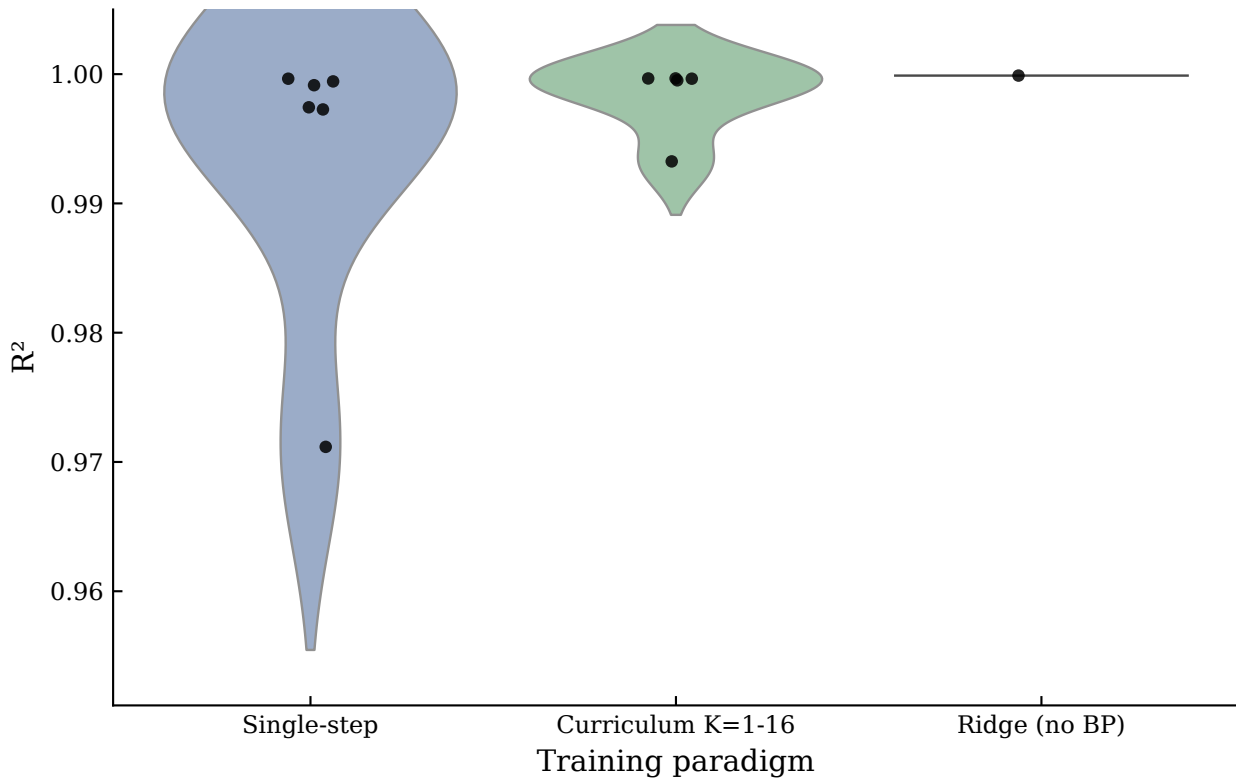
MG — R^2 by Training Paradigm
