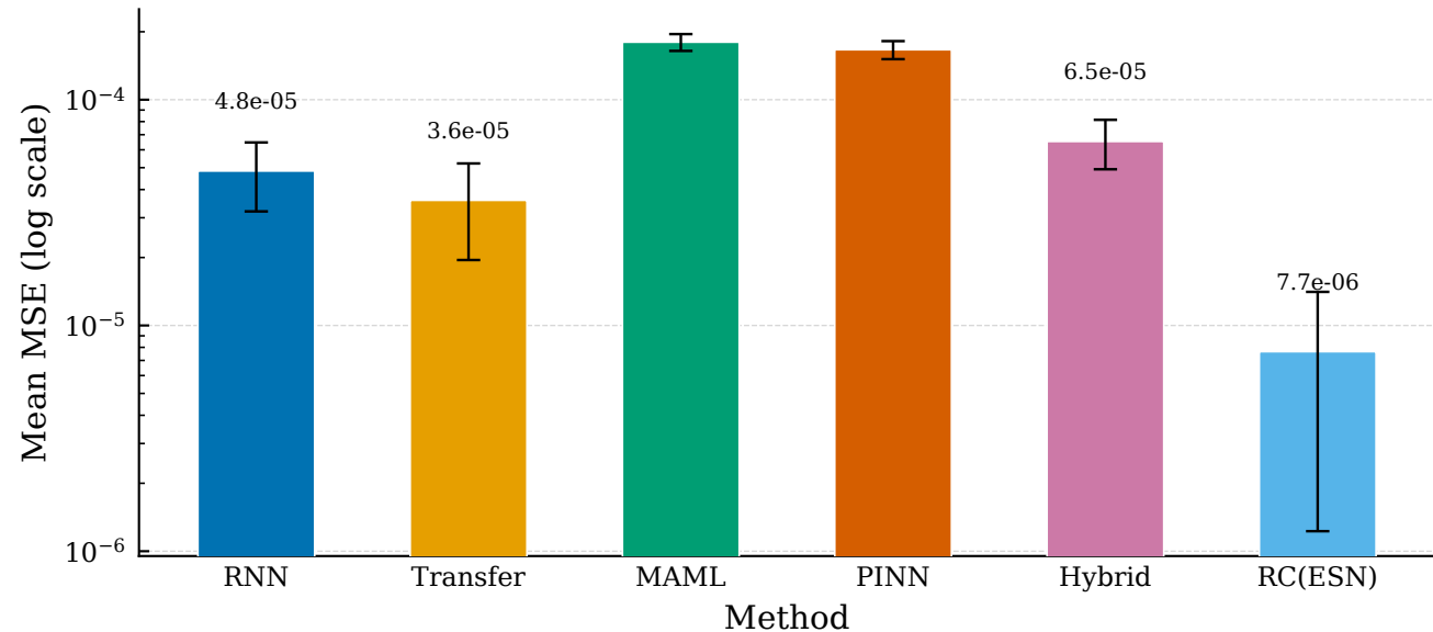
MG — Mean MSE Across 25 Random ICs
