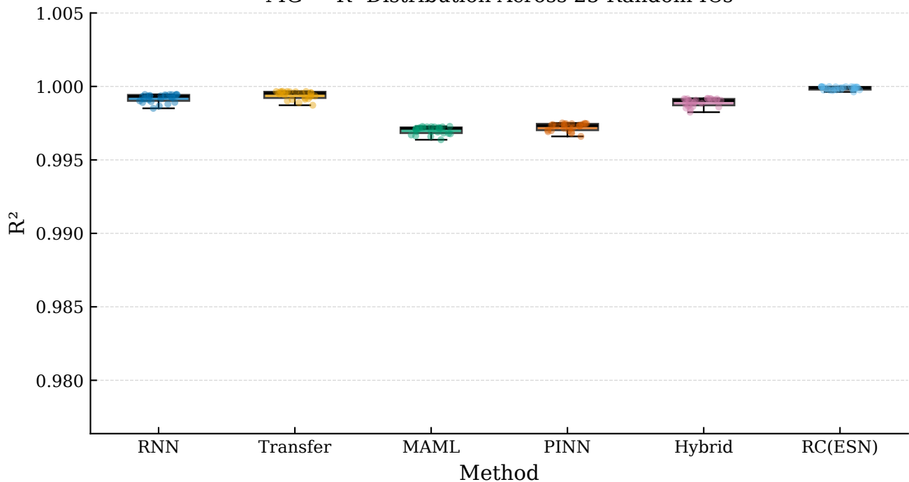
MG — R^2 Distribution Across 25 Random ICs
