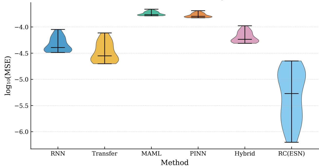
MG — MSE Distribution Shape ( \log_{10} scale)
