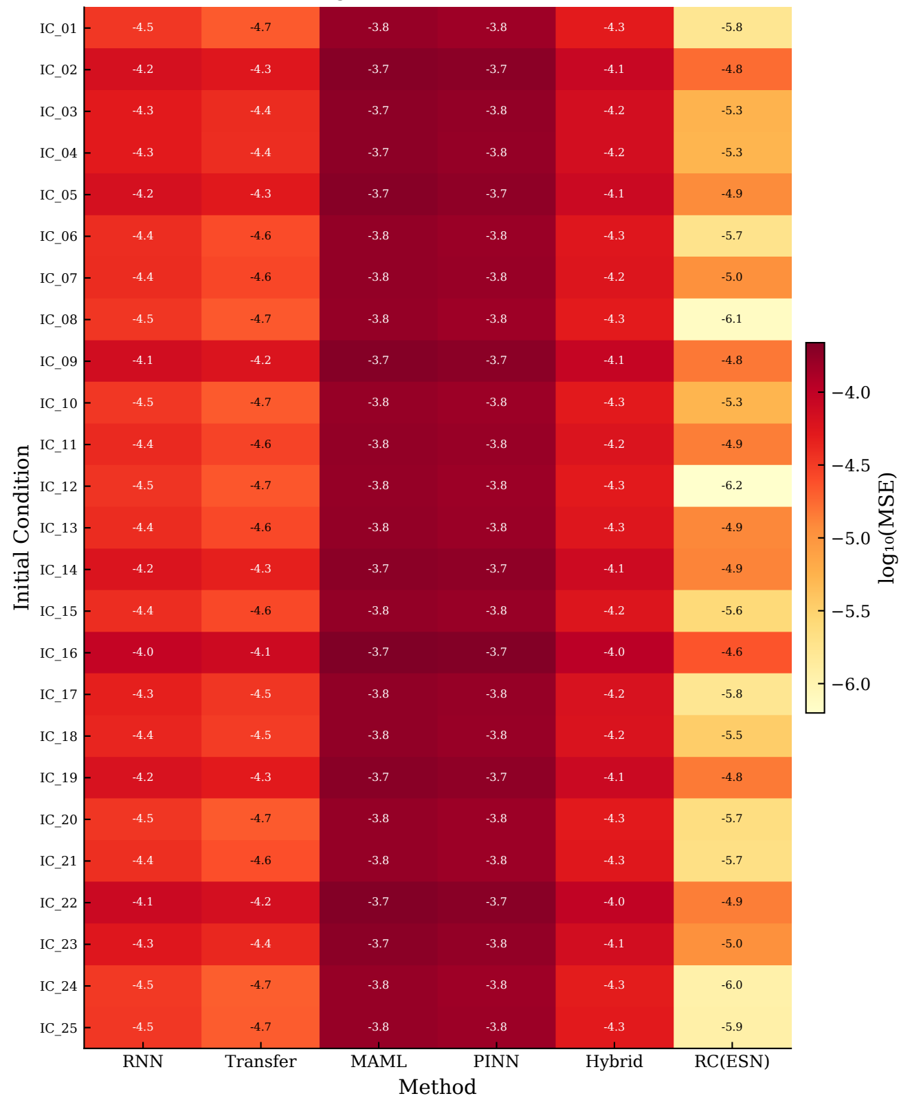
MG — \log_{10}(\text{MSE}) per IC and Method
