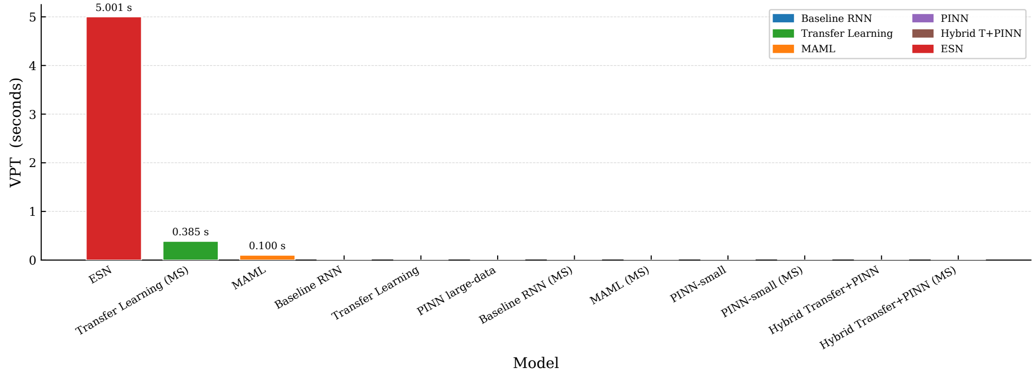
Lorenz — Valid Prediction Time in Seconds ( \lambda_1 \approx 0.905 )
