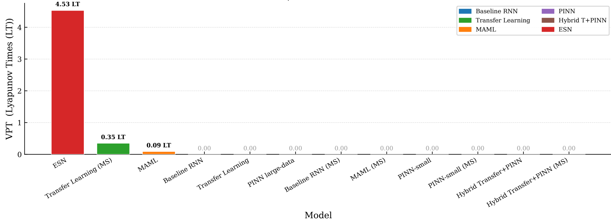
Lorenz — Valid Prediction Time [Lyapunov Times (LT)] \lambda_1 \approx 0.905 | NRMSE threshold = 0.4
