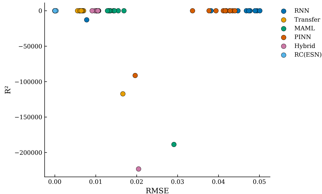
Lorenz — RMSE vs R^2 : All Method \times IC (stable ICs)
