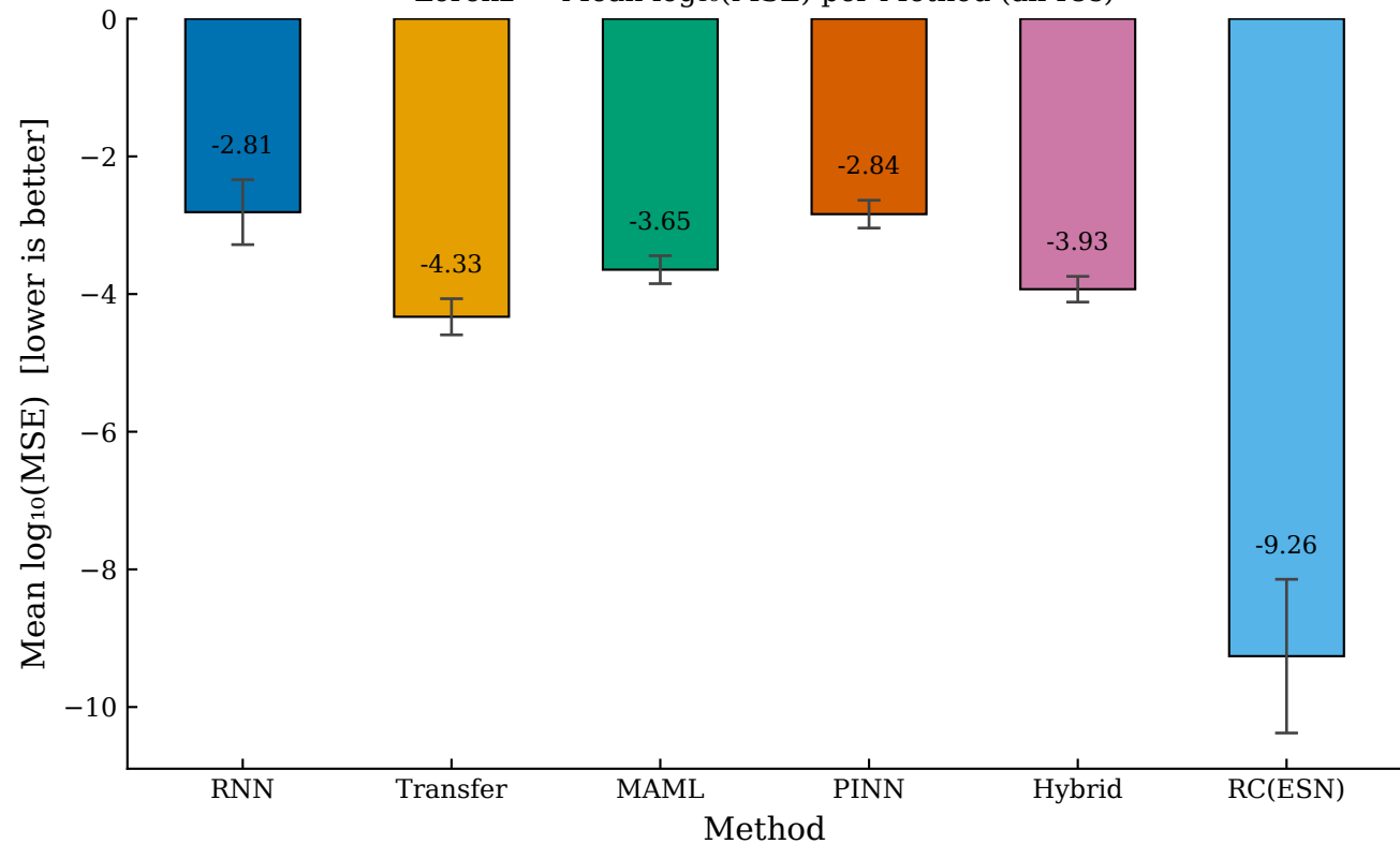
Lorenz — Mean \log_{10}(\text{MSE}) per Method (all ICs)
