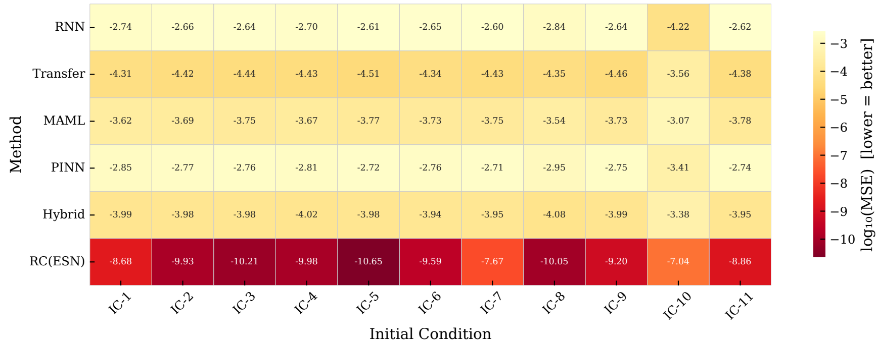
Lorenz — \log_{10}(\text{MSE}) Heatmap: Method \times IC [lower = better]
