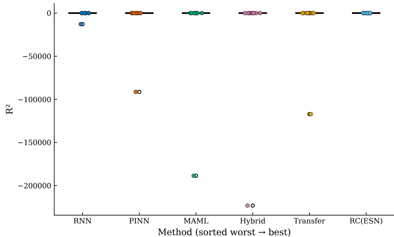
Lorenz — R 2 Distribution (stable ICs)
