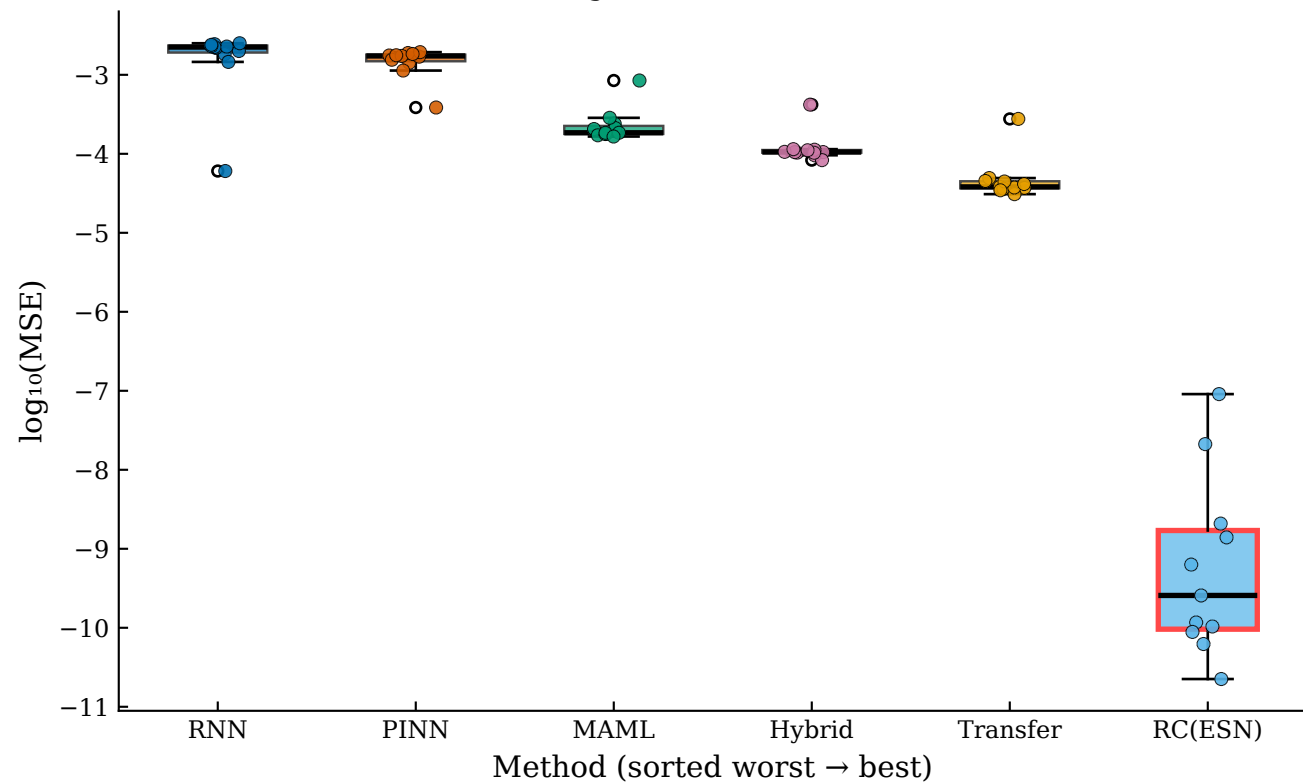
Lorenz — \log_{10}(\text{MSE}) Distribution (all ICs)
