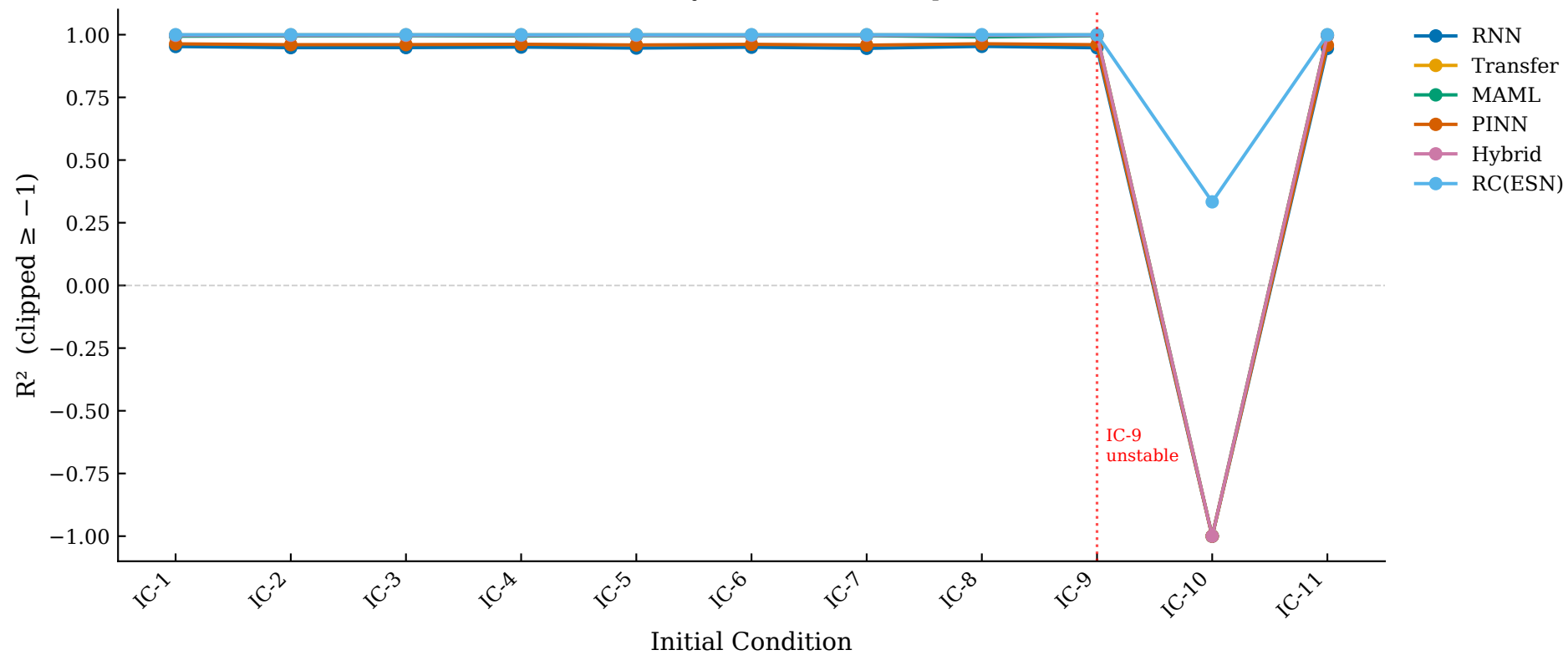
Lorenz — R 2 Sensitivity to Initial Condition per Method
