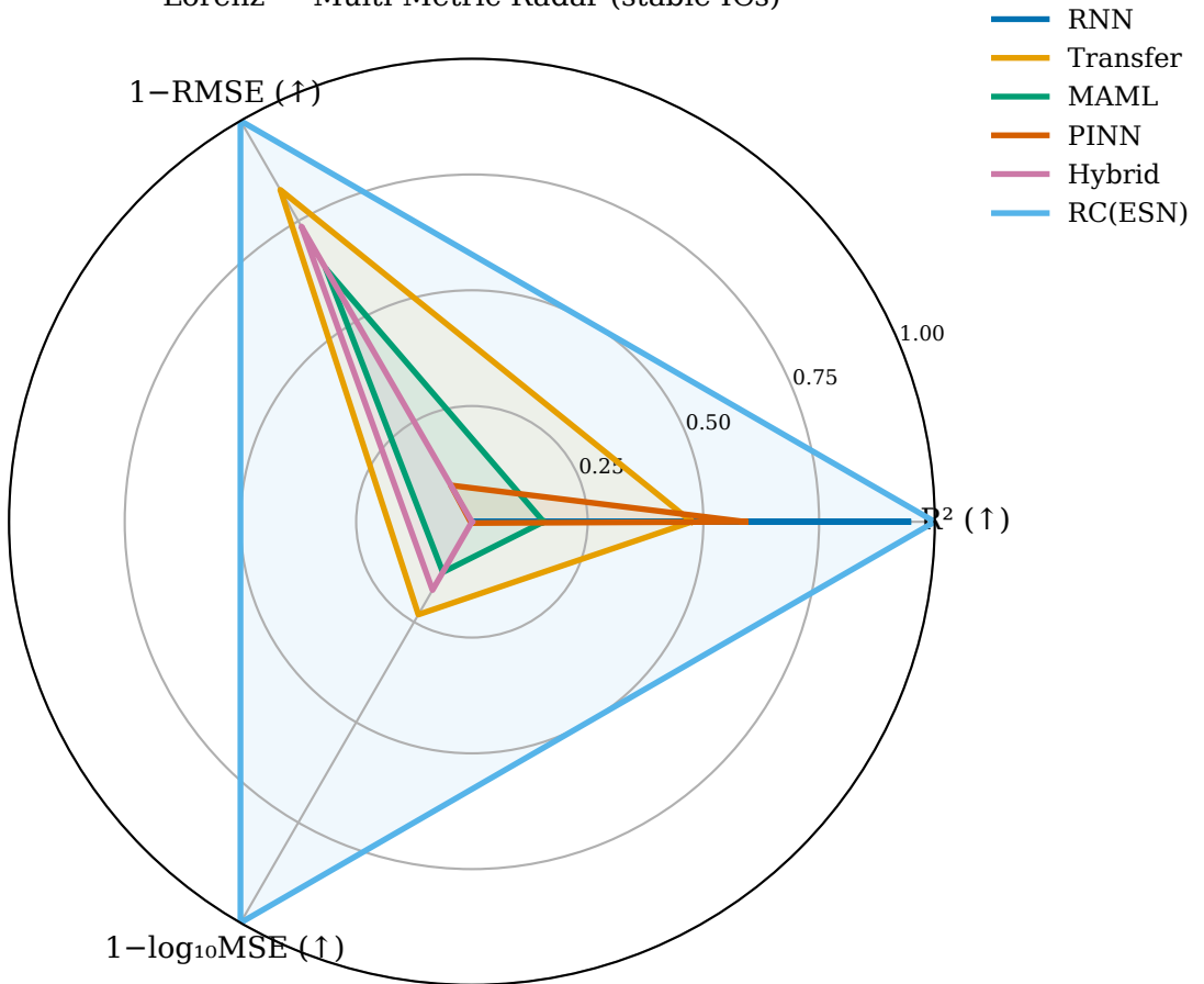
Lorenz — Multi-Metric Radar (stable ICs)
