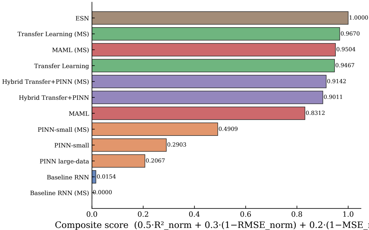
Lorenz — Composite Score Leaderboard
