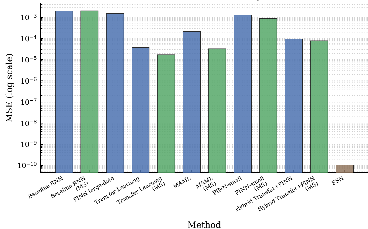
Lorenz — MSE: All Variants (log scale)
