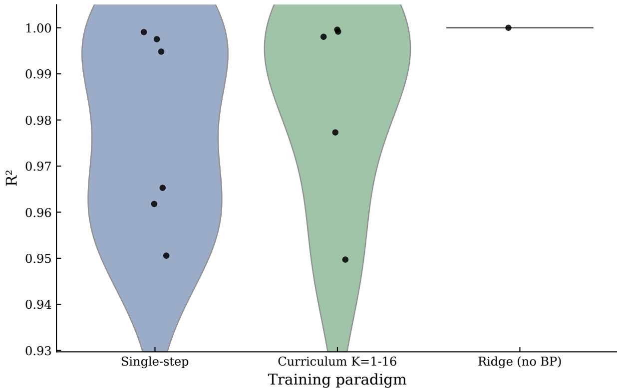
Lorenz — R^2 by Training Paradigm
