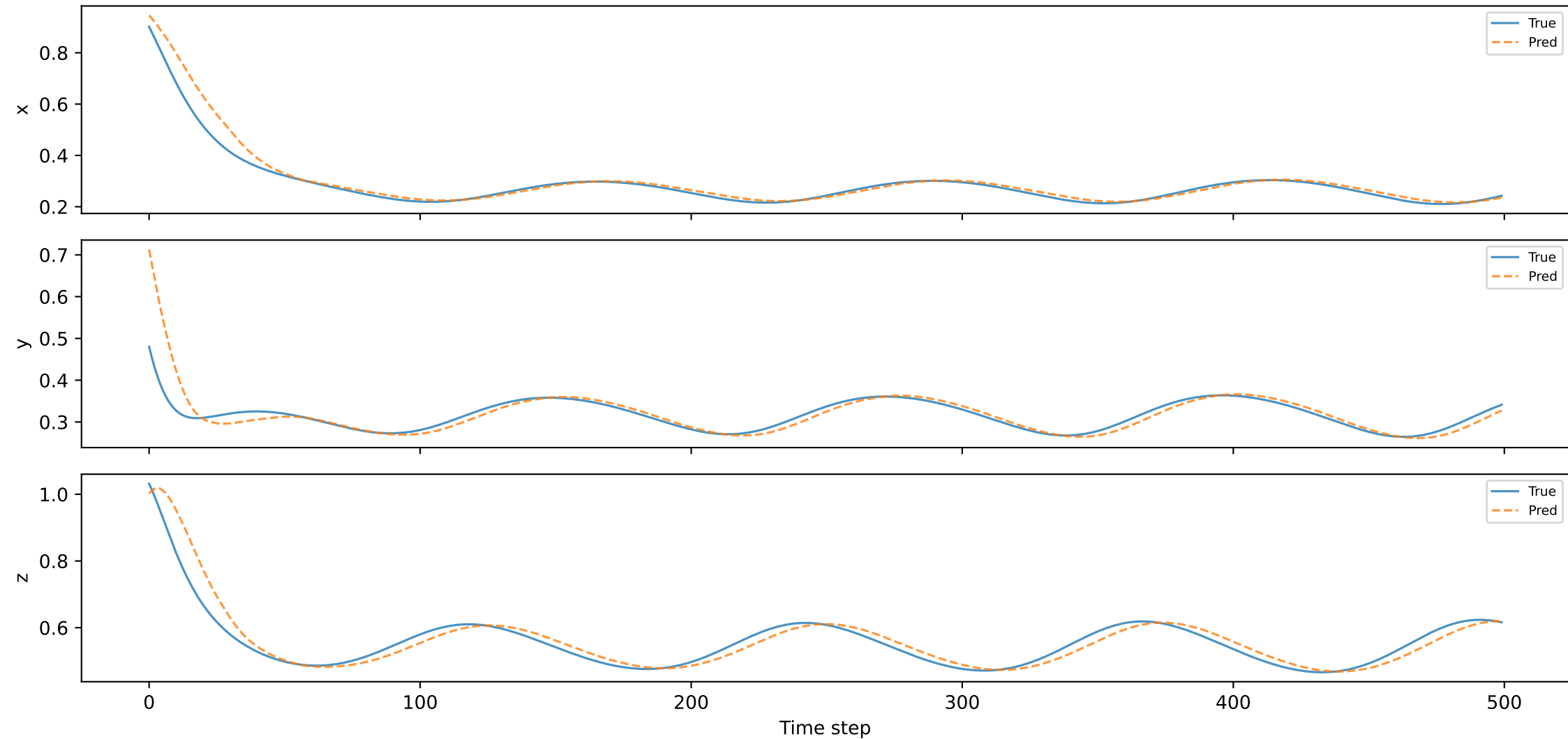
Baseline RNN (orig)
