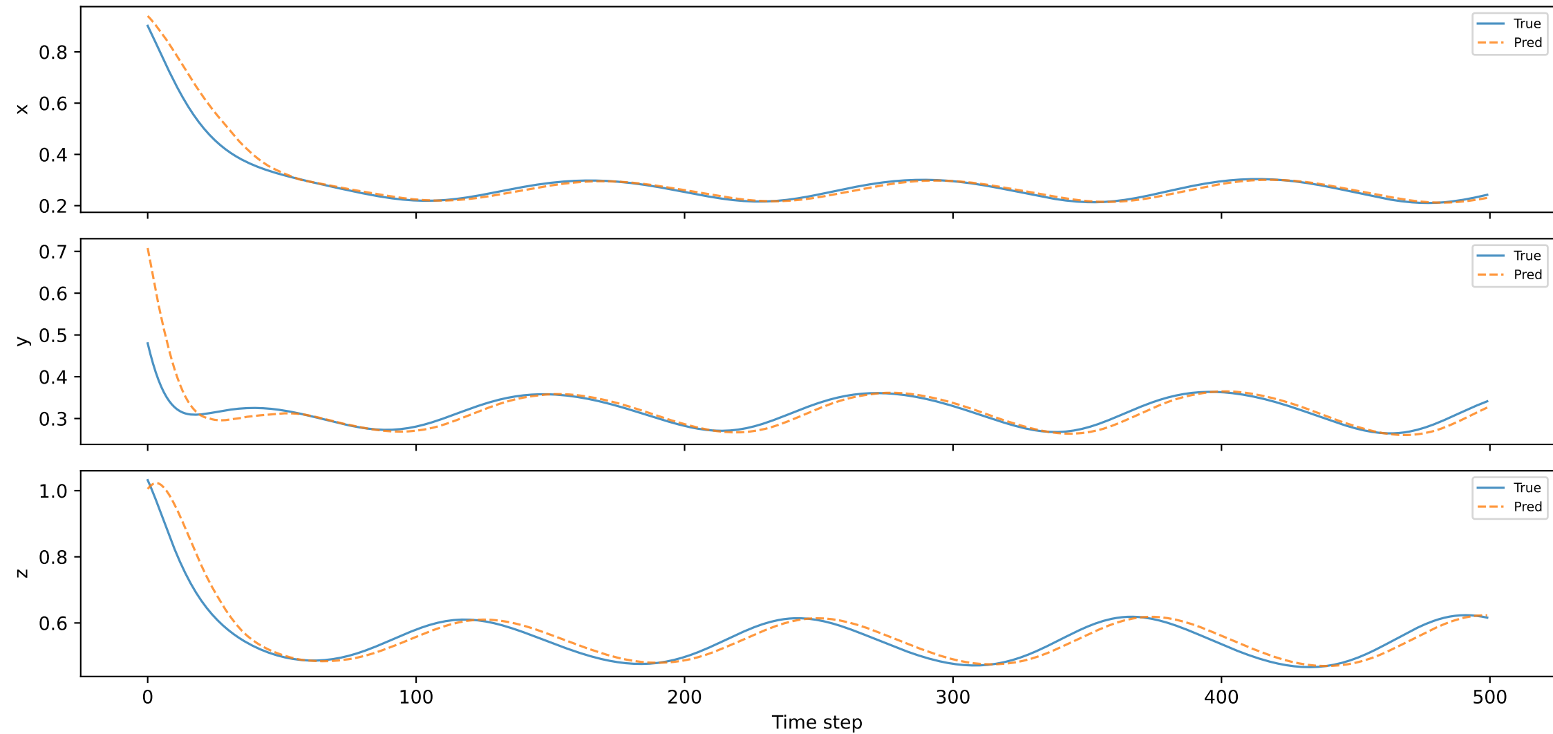
Baseline RNN - MS
