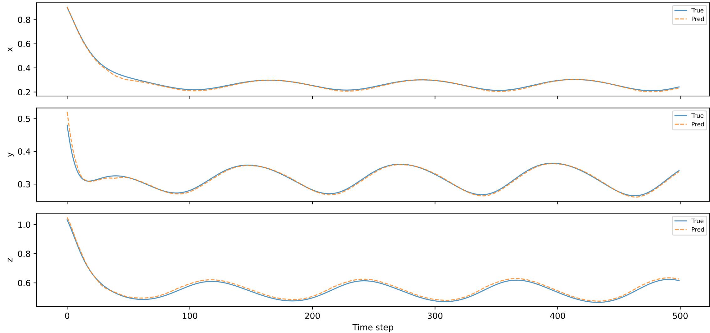
Transfer Learning - MS
