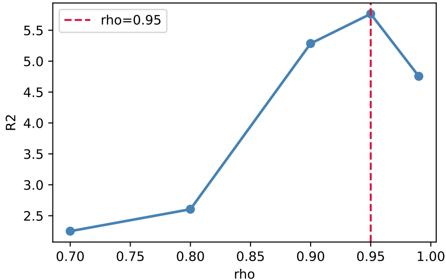
ESN R2 vs Spectral Radius
