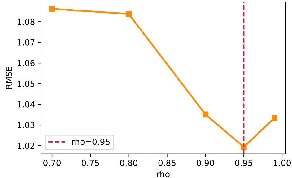
ESN RMSE vs Spectral Radius
