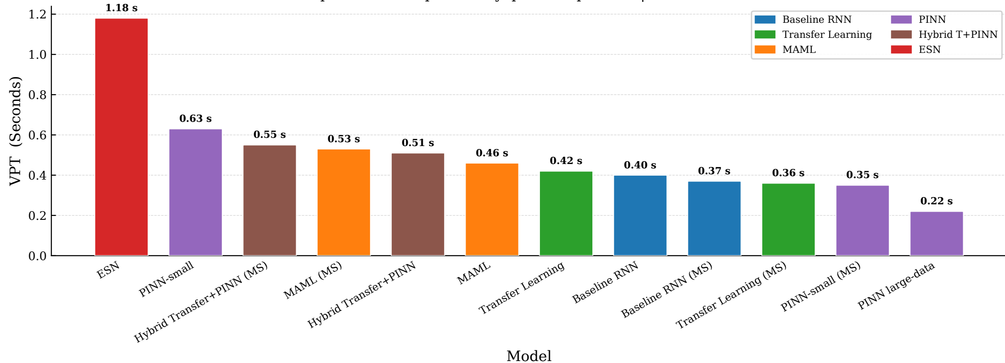
Duffing — Valid Prediction Time [Seconds] conservative periodic — no positive Lyapunov exponent | NRMSE threshold = 0.4
