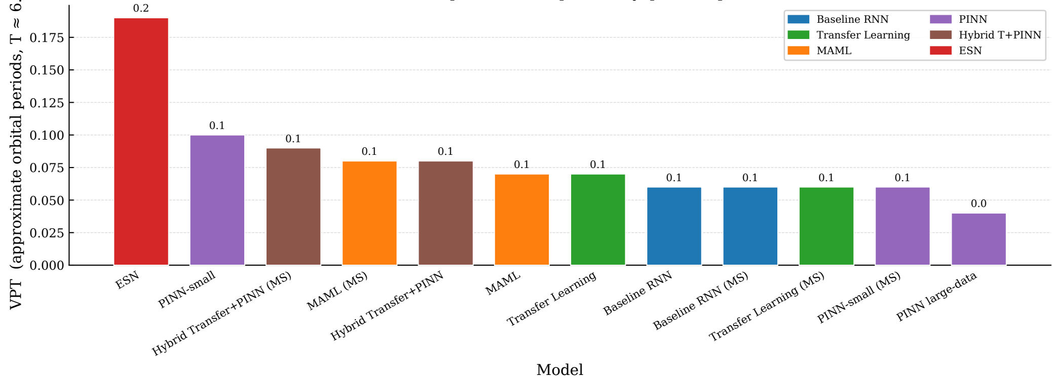
Duffing — Valid Prediction Time in Orbital Periods (conservative periodic — no positive Lyapunov exponent)
