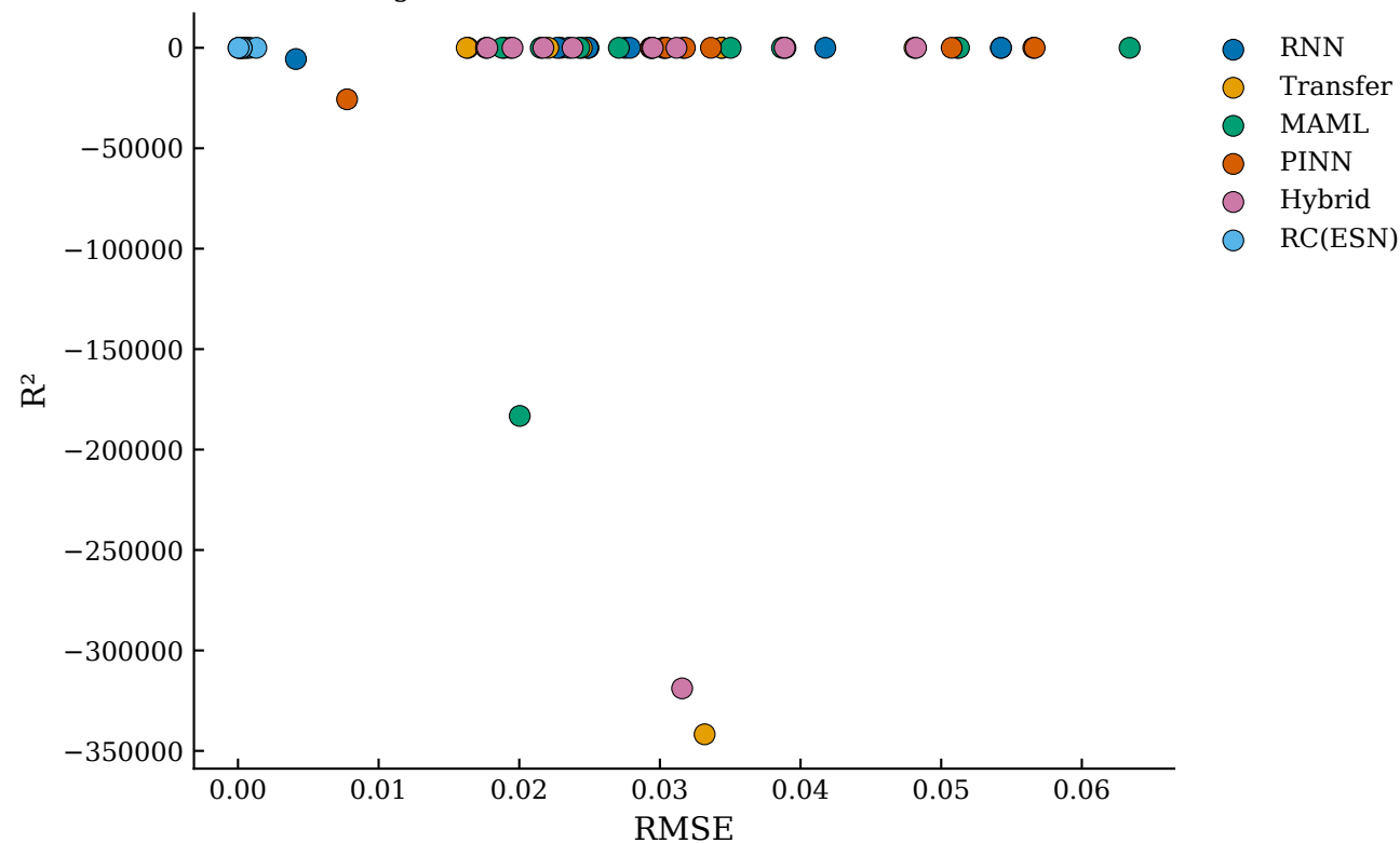
Duffing — RMSE vs R^2 : All Method \times IC (stable ICs)
