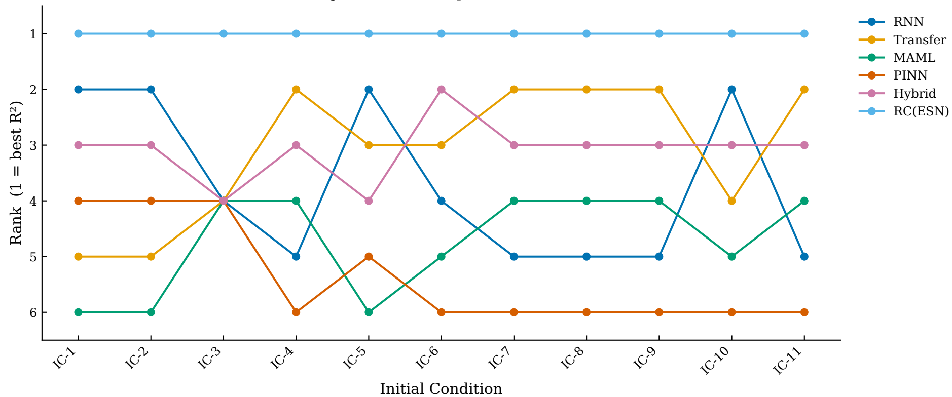
Duffing — Method Rank per Initial Condition
