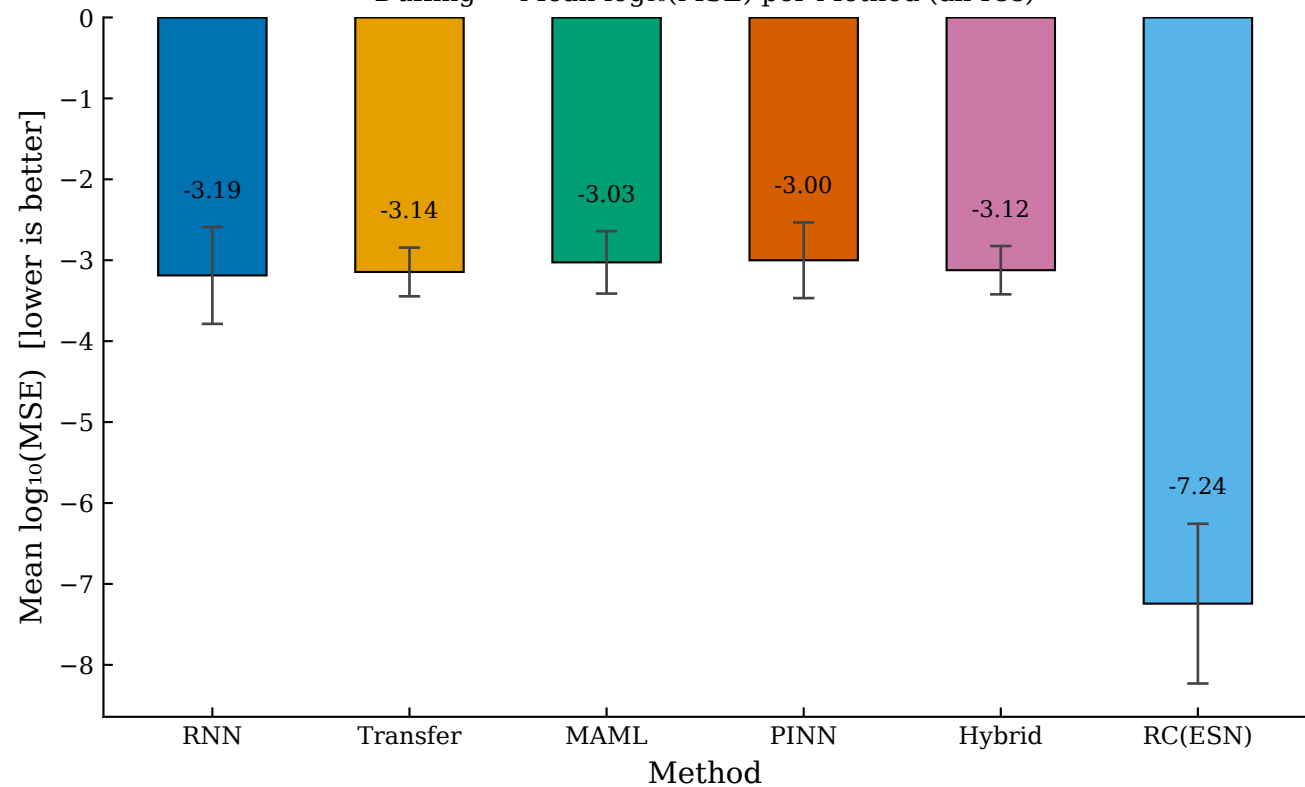
Duffing — Mean \log_{10}(\text{MSE}) per Method (all ICs)
