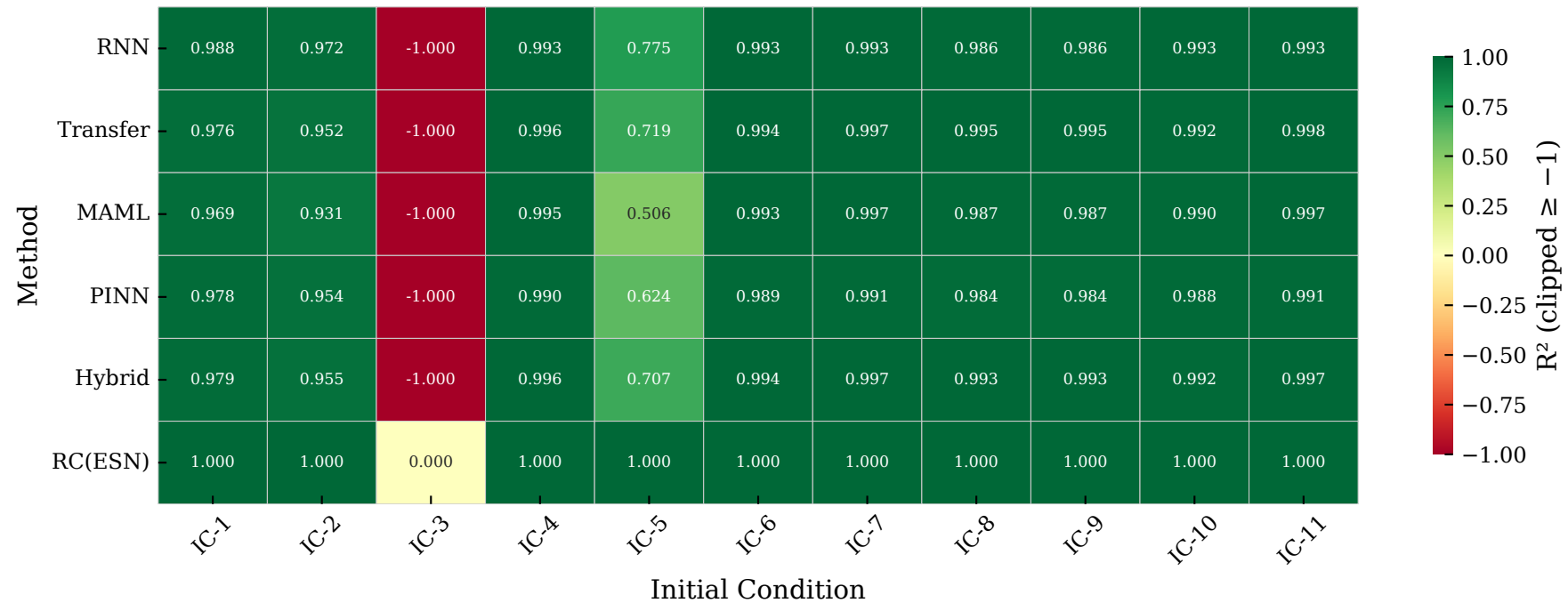
Duffing — R 2 Heatmap: Method × IC
