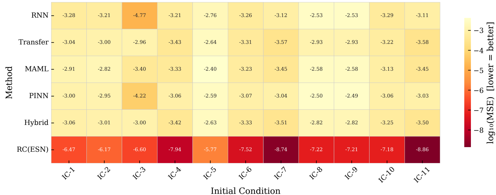
Duffing — \log_{10}(\text{MSE}) Heatmap: Method \times IC [lower = better]
