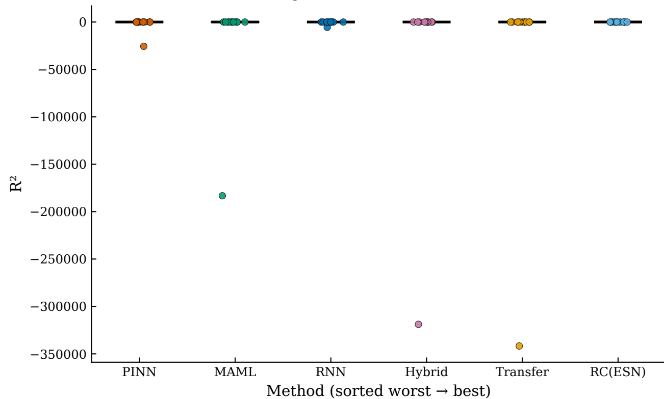
Duffing — R^2 Distribution (stable ICs)
