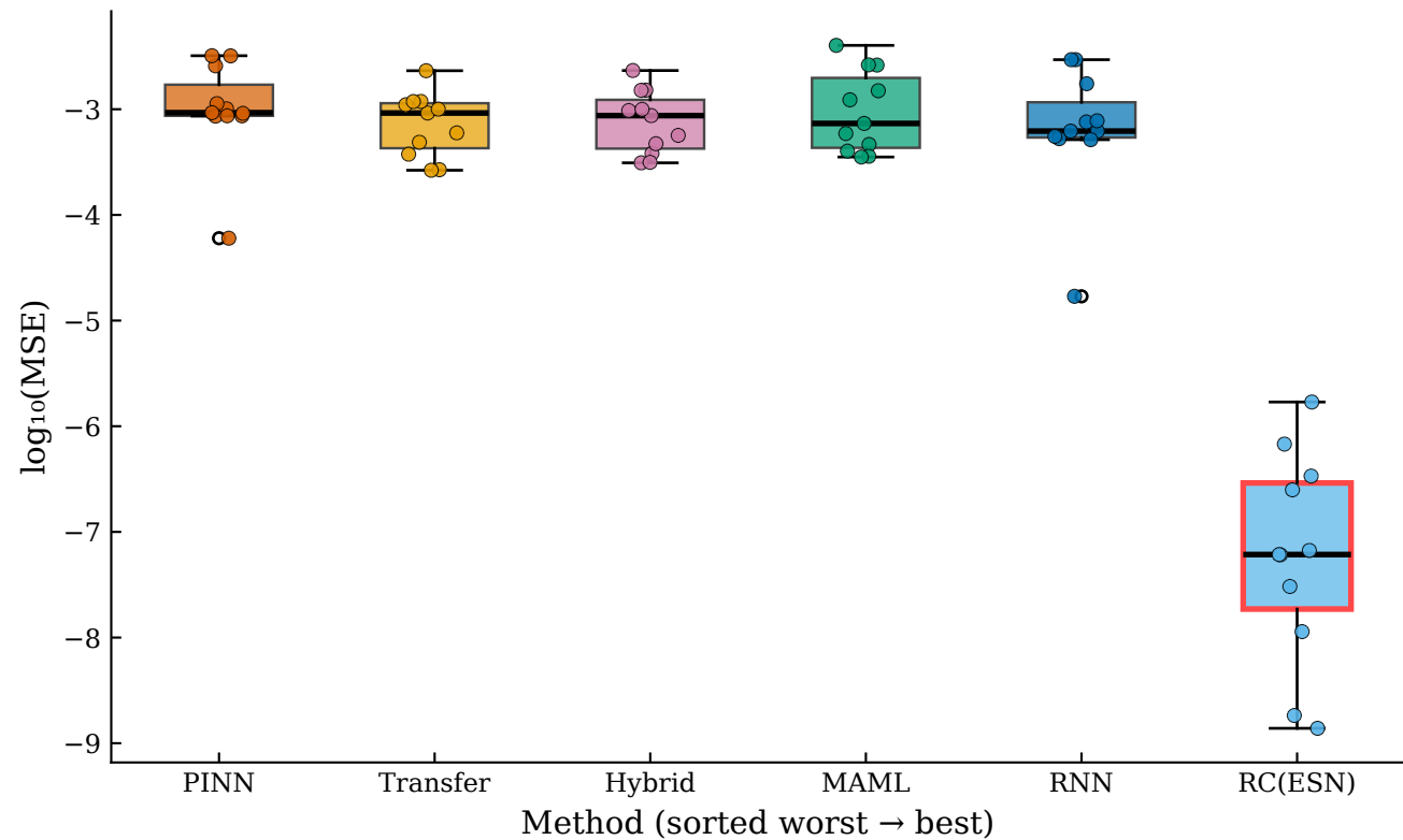
Duffing — \log_{10}(\text{MSE}) Distribution (all ICs)
