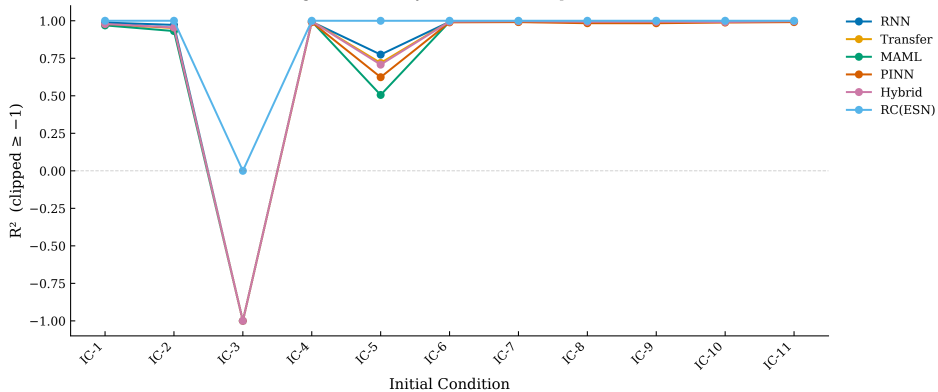
Duffing — R 2 Sensitivity to Initial Condition per Method
