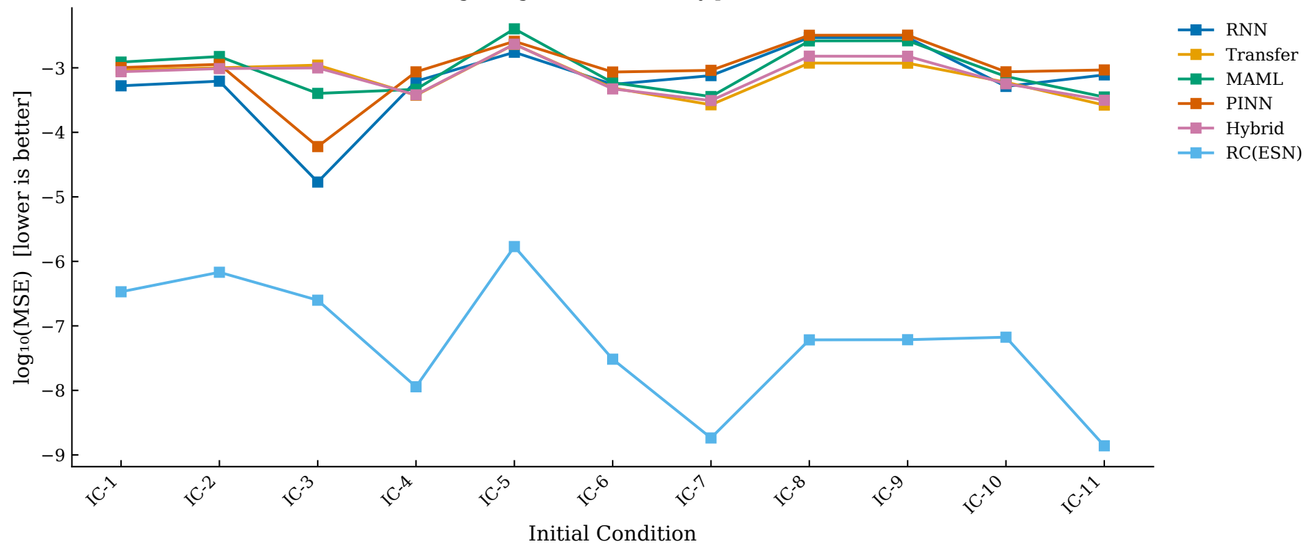
Duffing — \log_{10}(\text{MSE}) Sensitivity per Method
