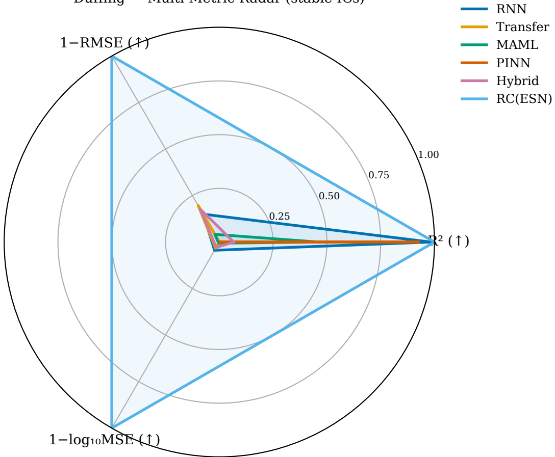
Duffing — Multi-Metric Radar (stable ICs)
