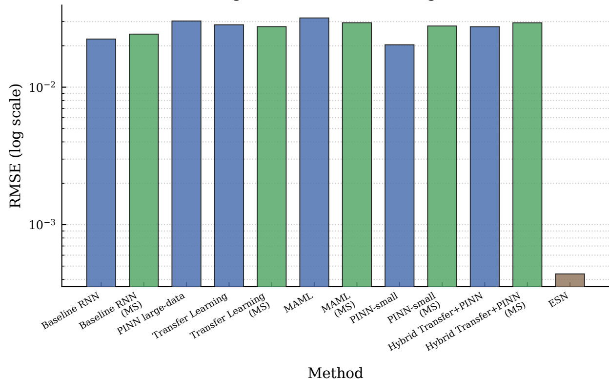
Duffing — RMSE: All Variants (log scale)
