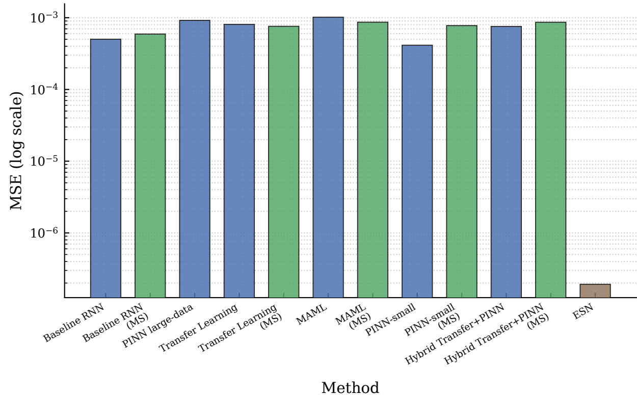
Duffing — MSE: All Variants (log scale)
