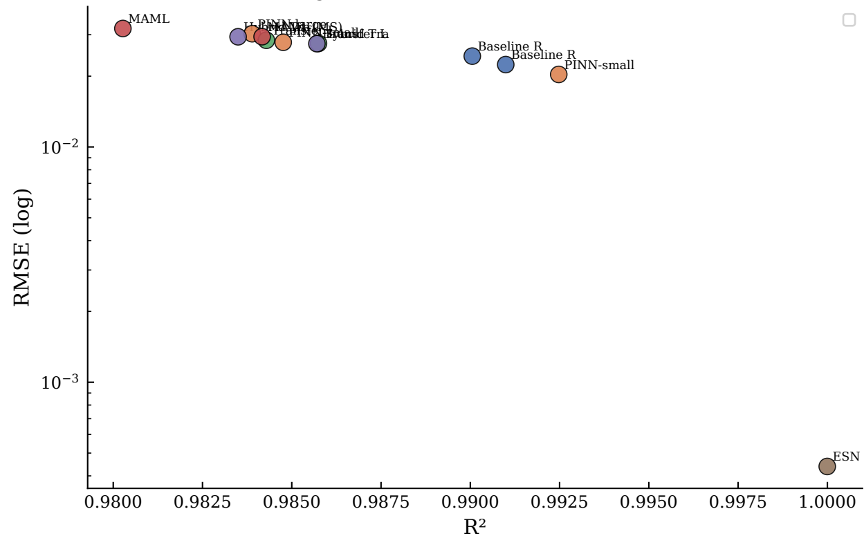
Duffing — RMSE vs R^2 with Pareto Frontier
