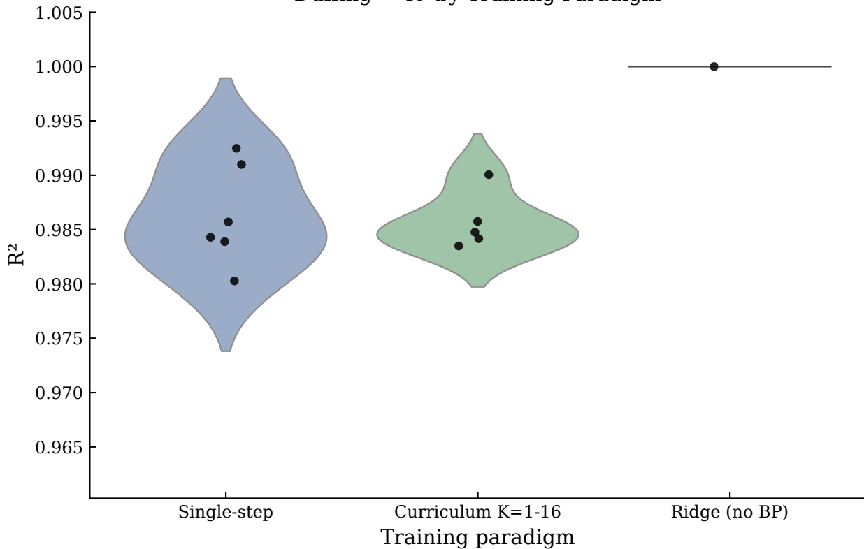
Duffing — R^2 by Training Paradigm
