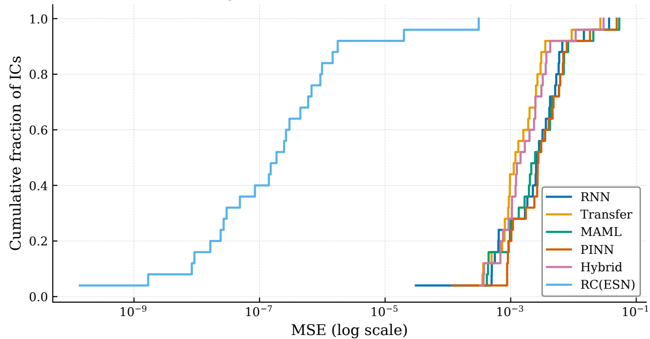
Duffing — Empirical CDF of MSE per Method
